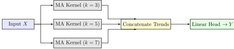
Figure 4.6: The Multi-Kernel DLinear extraction phase. Multiple kernels capture volatility at different frequencies.
