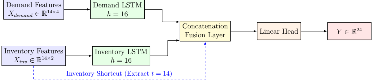
Figure 4.4: The Dual-Stream Inventory Shortcut LSTM Architecture. Notice the dashed shortcut preserving the t = 14 state.
