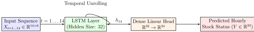
Figure 4.3: The Canonical LSTM processing pipeline for 24-hour stockout prediction.
