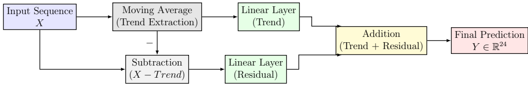
Figure 4.5: The Standard DLinear Architecture. Trend and residual mapped via independent linear layers.
